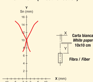
MOD. FDL311 (Riflessione diretta) TYPES FDL311 (Direct reflection)
