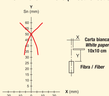
MOD. FDL010 - FDL310 (Riflessione diretta) TYPES FDL010 - FDL310 (Direct reflection)
