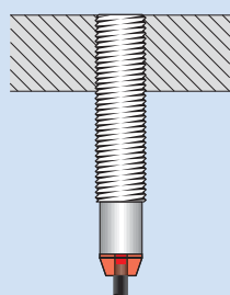
Flush mounting
