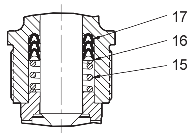
1" Stem Seal Construction
