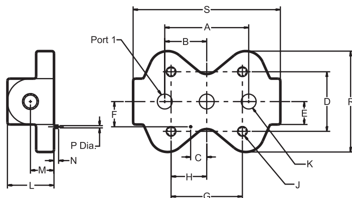
3-Way Sub-Base
